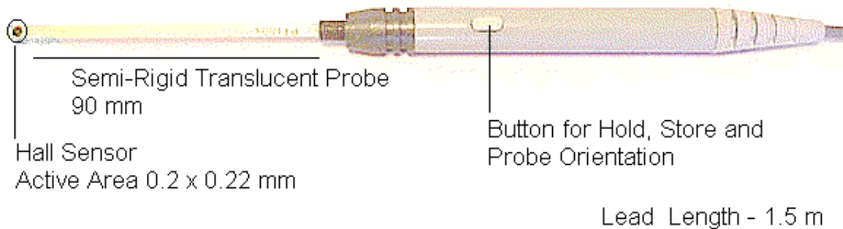
Transverse Hall Probe - 230 mm
